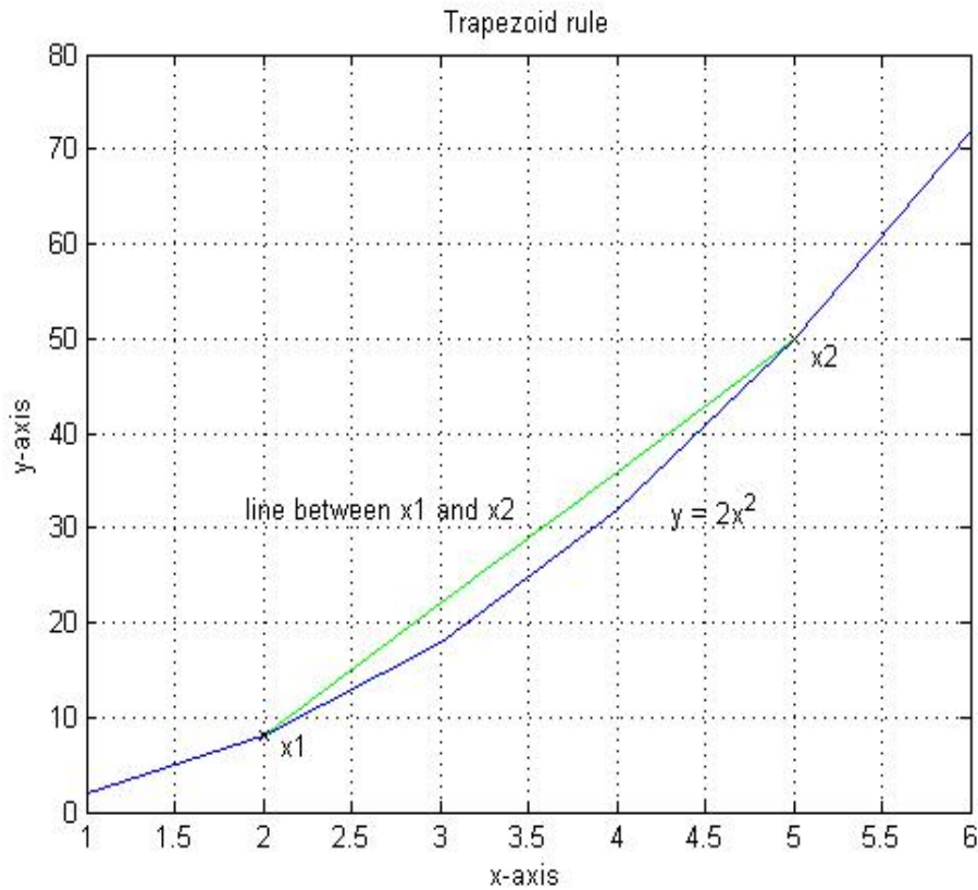
Figure 1 Trapezoid Rule
