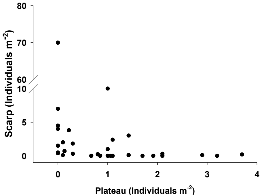
Figure 4. Distribution of the 32 sponge species recorded at GRNMS and J Reef. Each point represents the mean number of individuals m -2 for each species. The density of each sponge species on the scarp is plotted against the density for that species on the plateau. N = 104 quadrats of 0.25 m 2 for both species density on the scarp and for the plateau.
