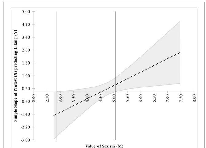
FIGURE 7 | The JN graph for the model relating Liking to Protesting, Sexism, and their interaction. Notice the effect of Protesting on Liking is significant only for high levels of Sexism.
