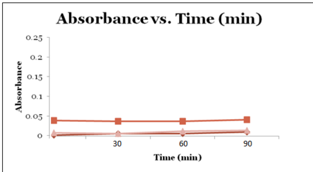
Graph 6. Tris-Indole with Chromium Chloride at 580 nm.
