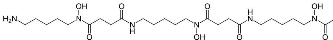
Figure 1: Desferrioxamine B
