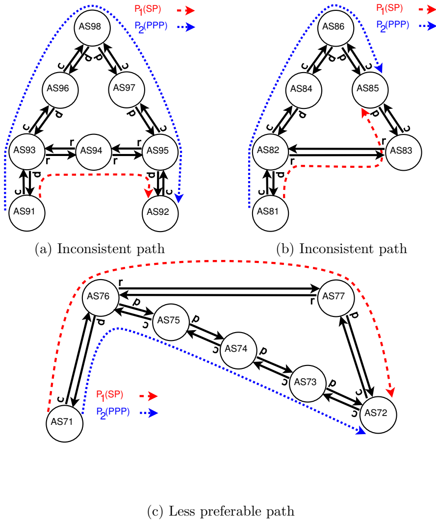
Figure 8: Policy Preferred Paths (PPP) algorithm compared to the Shortest Paths (SP) algorithm
