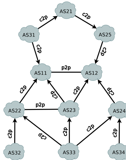
Figure 1: An illustrative AS-level Internet topology map consisting of 11 ASes (clouds) and 15 relations (links) among them.
