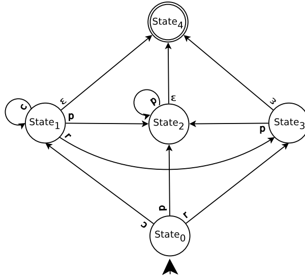
Figure 4: NFA- \epsilon recognizing valley-free AS paths
