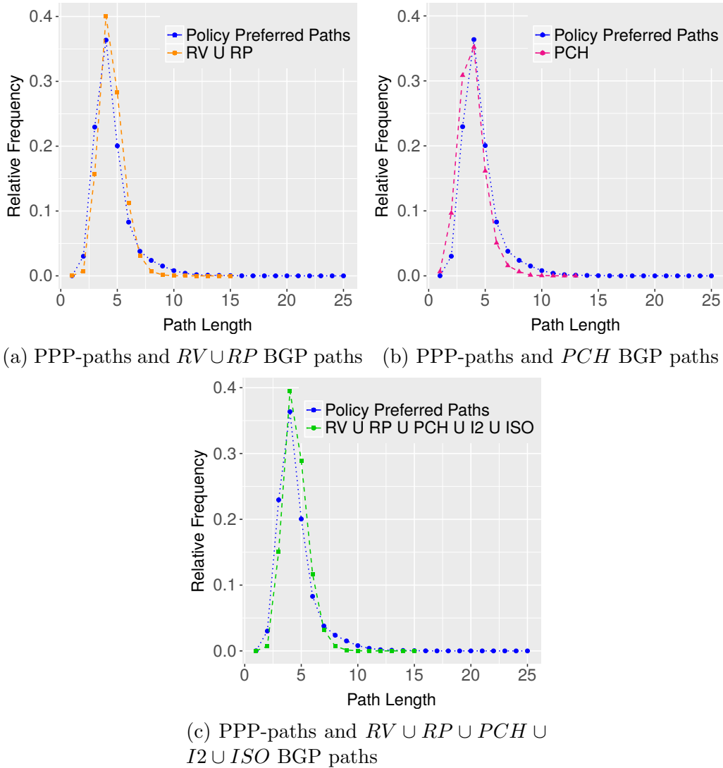
Figure 9: Relative path lengths comparison of PPP-paths and raw BGP paths
